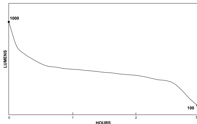
PERFORMANCE CURVE
